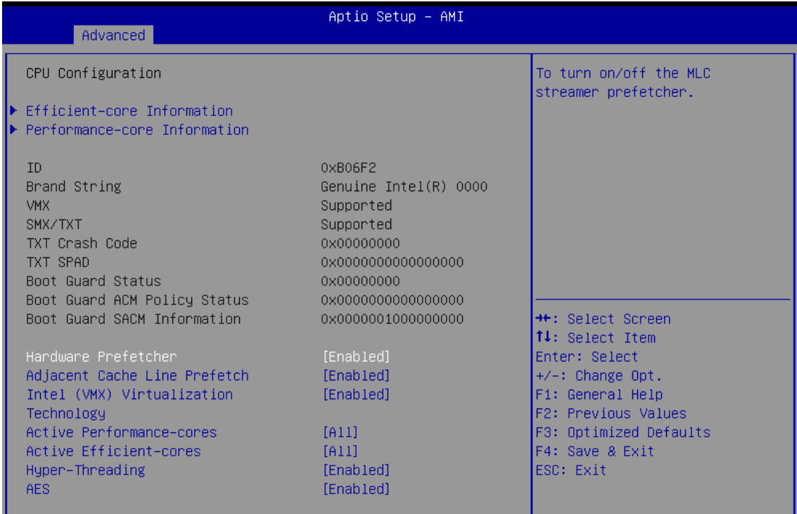
Figure 4-3-1 : CPU Configuration
