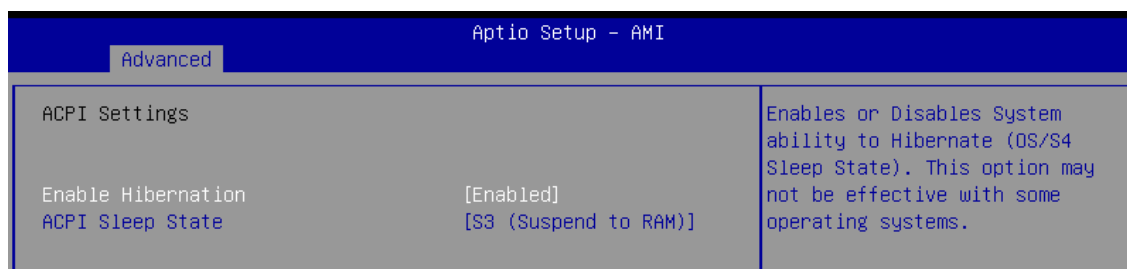
Figure 4-3-4 : ACPI Settings
